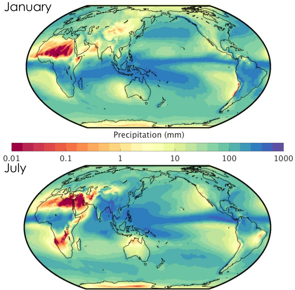
Figure 5.2: Average rainfall for January (top) and July (bottom) 1981 – 2010. Data source: ECMWF Interim Reanalysis, for 1981 – 2010 (Dee et al. 2011).
