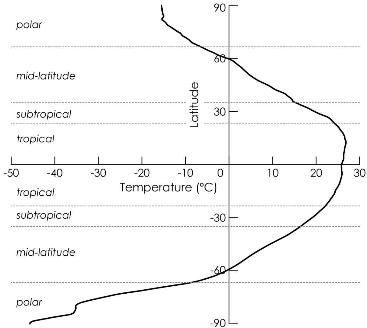
Figure 5.6 Temperature as a function of latitude (the North Pole is at the top; the South Pole at the bottom). Data source: ECMWF Interim Reanalysis, for 1981 – 2010
