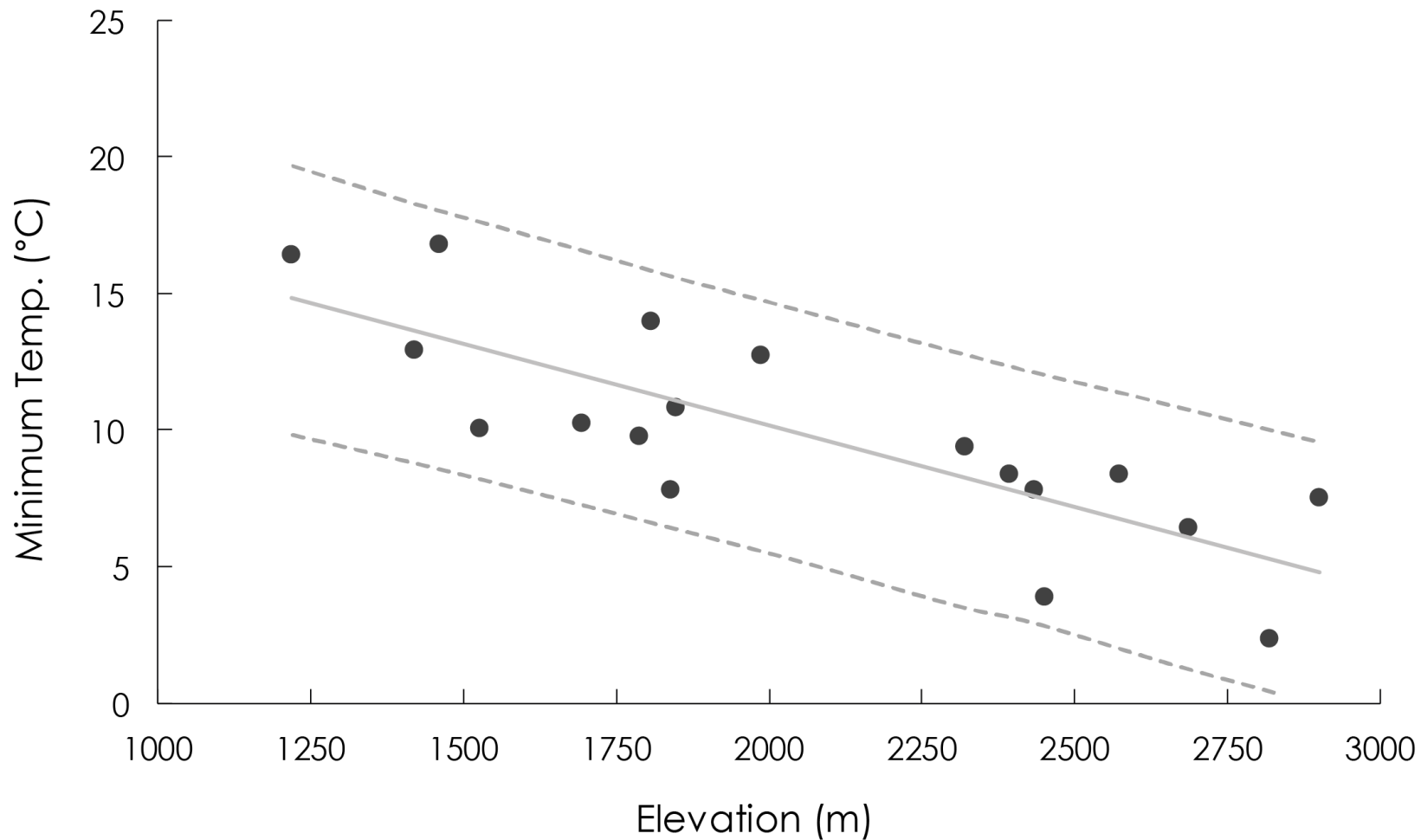
Figure 5.4 Climatological (1981–2010) monthly average minimum temperature (°C) as a function of elevation for 18 stations in the Ethiopian Highlands (locations shown in insert). Points indicate the lowest climatological monthly minimum temperature during the calendar year, with the solid line showing a least squares linear fit and dashed lines indicating the 95% confidence limits for predicted values
