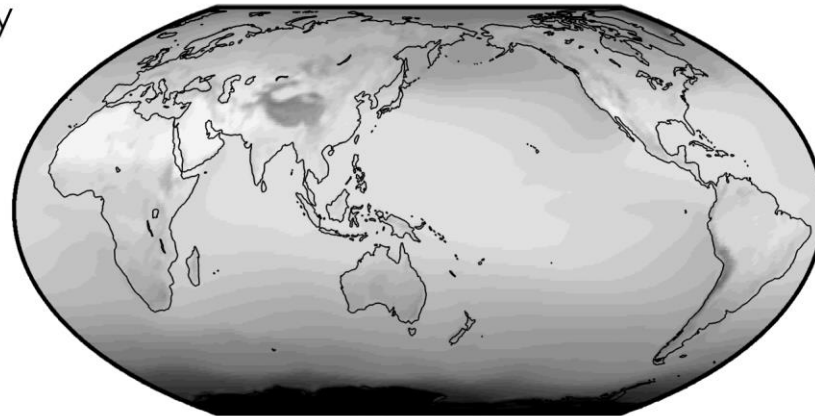
Figure 5.1: Average temperatures for January (top) and July (bottom) 1981 – 2010. Data source: ECMWF Interim Reanalysis, for 1981 – 2010 (Dee et al. 2011).
