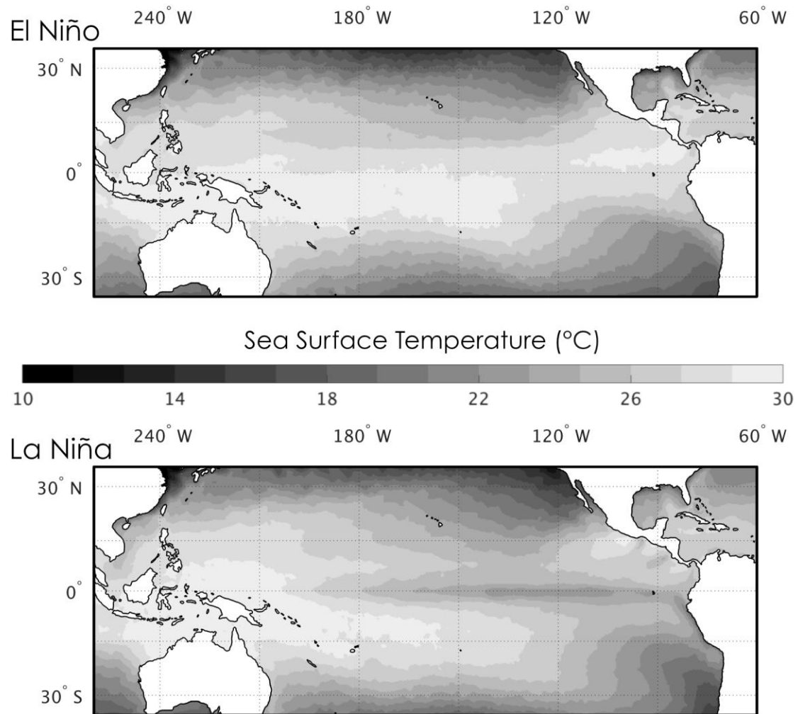
Figure 5.13 Sea-surface temperatures during (top) a strong El Niño event (Dec 1997 – Feb 1998), and (bottom) a strong La Niña event (Dec 1998 – Feb 1999). Data source: OISST2(Reynolds et al. 2007).
